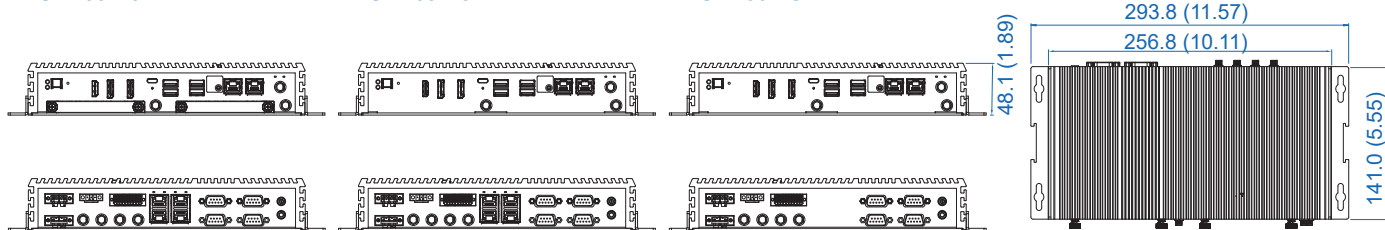
ECS-4700-PoER
